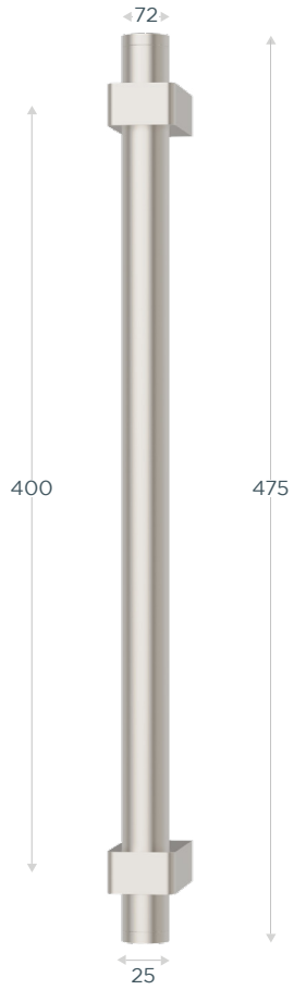
Barrel Pull Handle - PS1001
