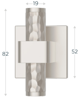
Projection: 59mm | 52mm Square Flat Rose
