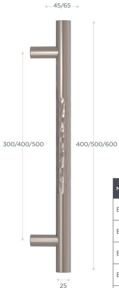
Barrel Pull Handle - PH7813
